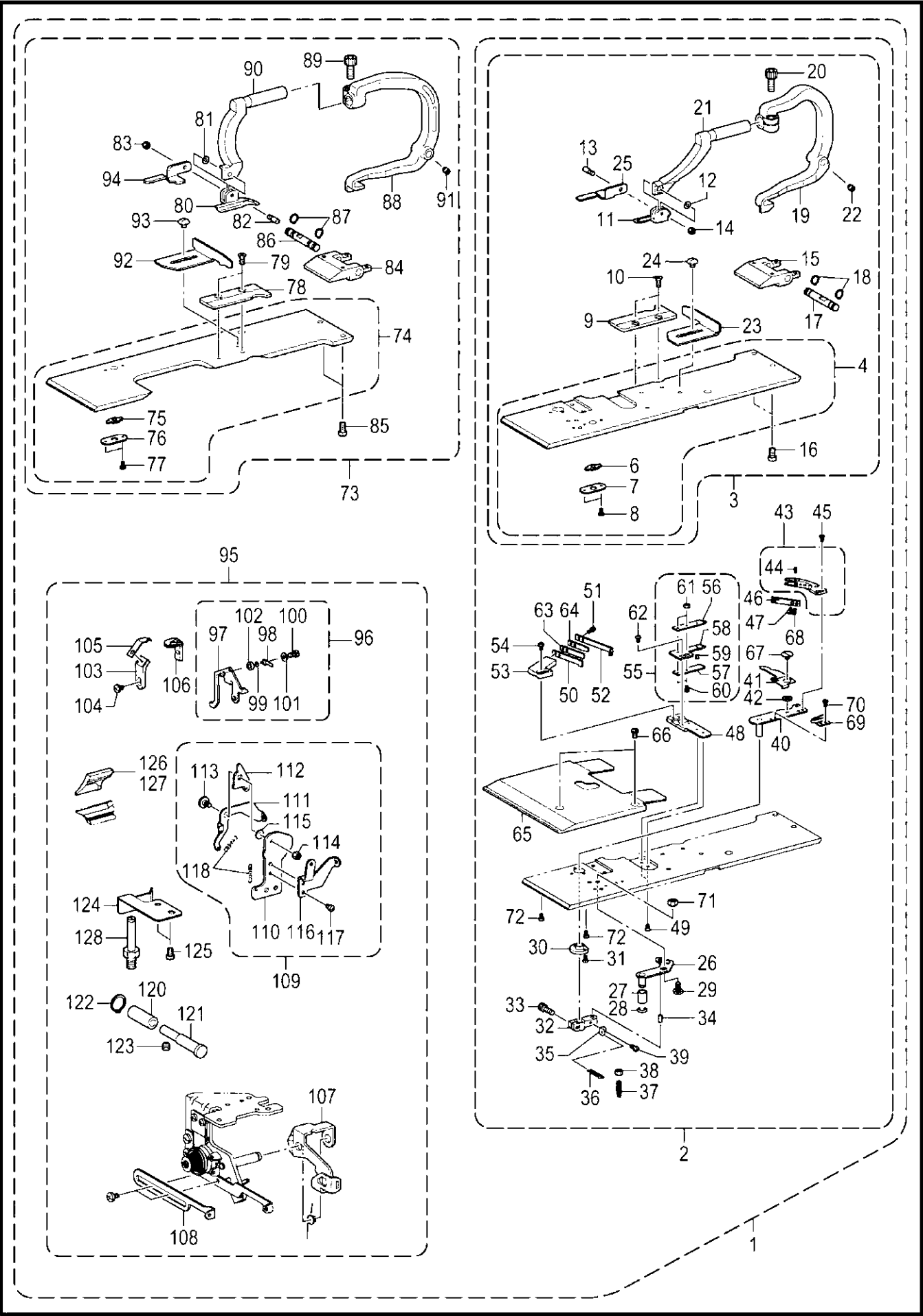
AA4. 附属装置 / Attachment set
